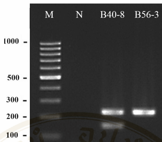
Figure 1. Duplex PCR. M, GeneRuler 100-bp DNA ladder (Thermo Fisher Scientific); N, no-template control; B40-8 and B56-3 DNA templates.
