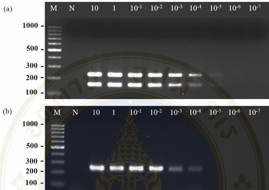
Figure 2. DNA detection limit with varying amounts of DNA template (ng) from B40-8 (a) and B56-3 (b). M, GeneRuler 100-bp DNA ladder (Thermo Fisher Scientific); N, no-template control.
